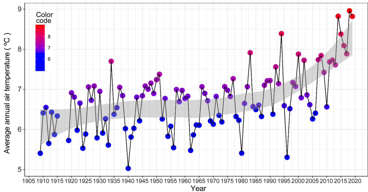
Abbildung 2: Average annual air temperature from 1909-2018 in Lunz am See.
