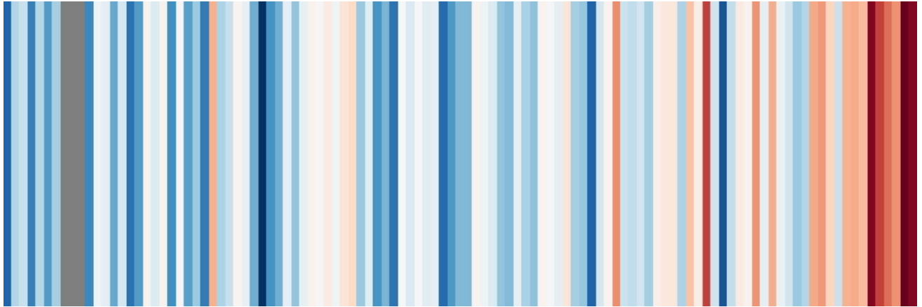
Figure 1: The “Lunz barcode” of climate change from 1909-2018.
